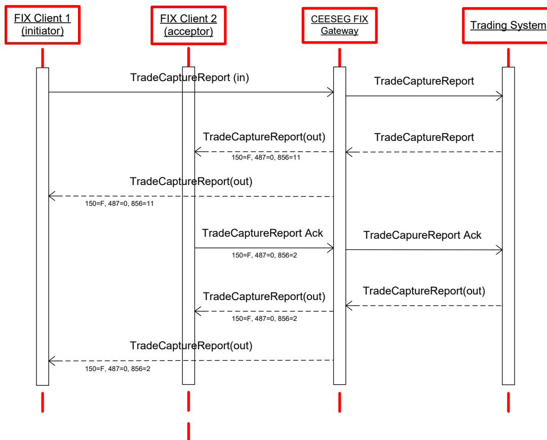
Figure 14 OTC Trade reporting message flow
