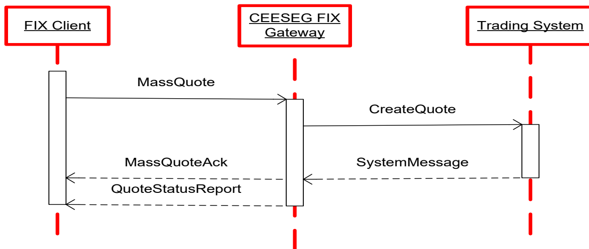
Figure 15 MassQuote message flow
