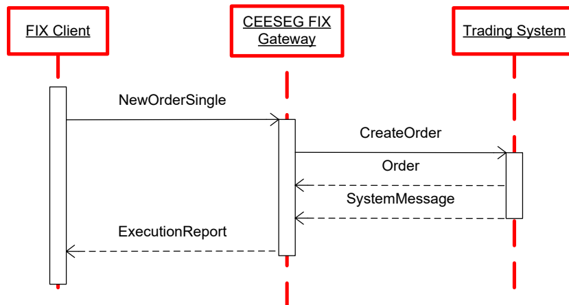
Figure 4 Order entry message flow
